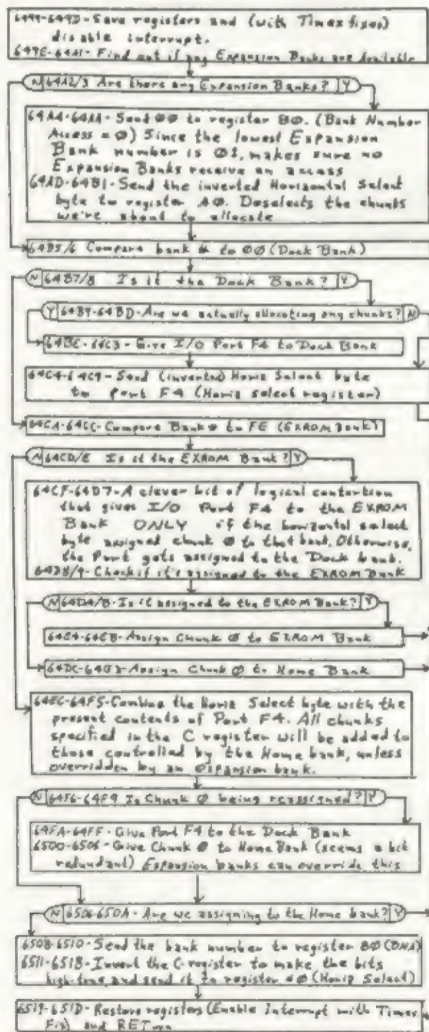
Flowchart 2. BANK_ENABLE in RAM Resident Code
